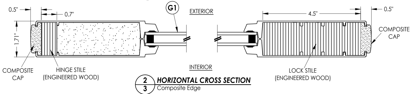
1 3 HORIZONTAL CROSS SECTION Wood Edge
