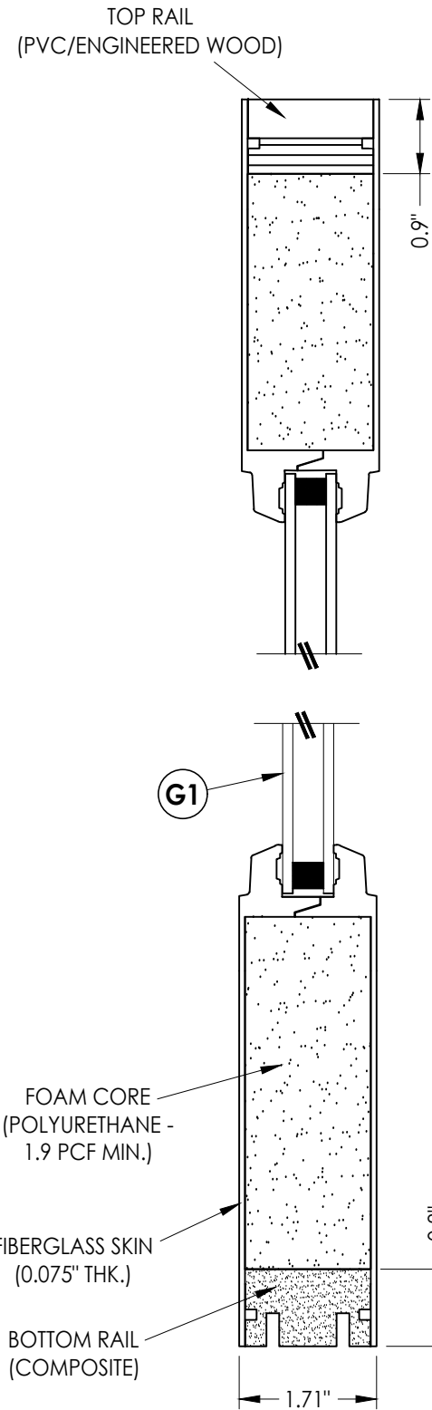
3 3 VERTICAL CROSS SECTION Wood or Composite Edge
